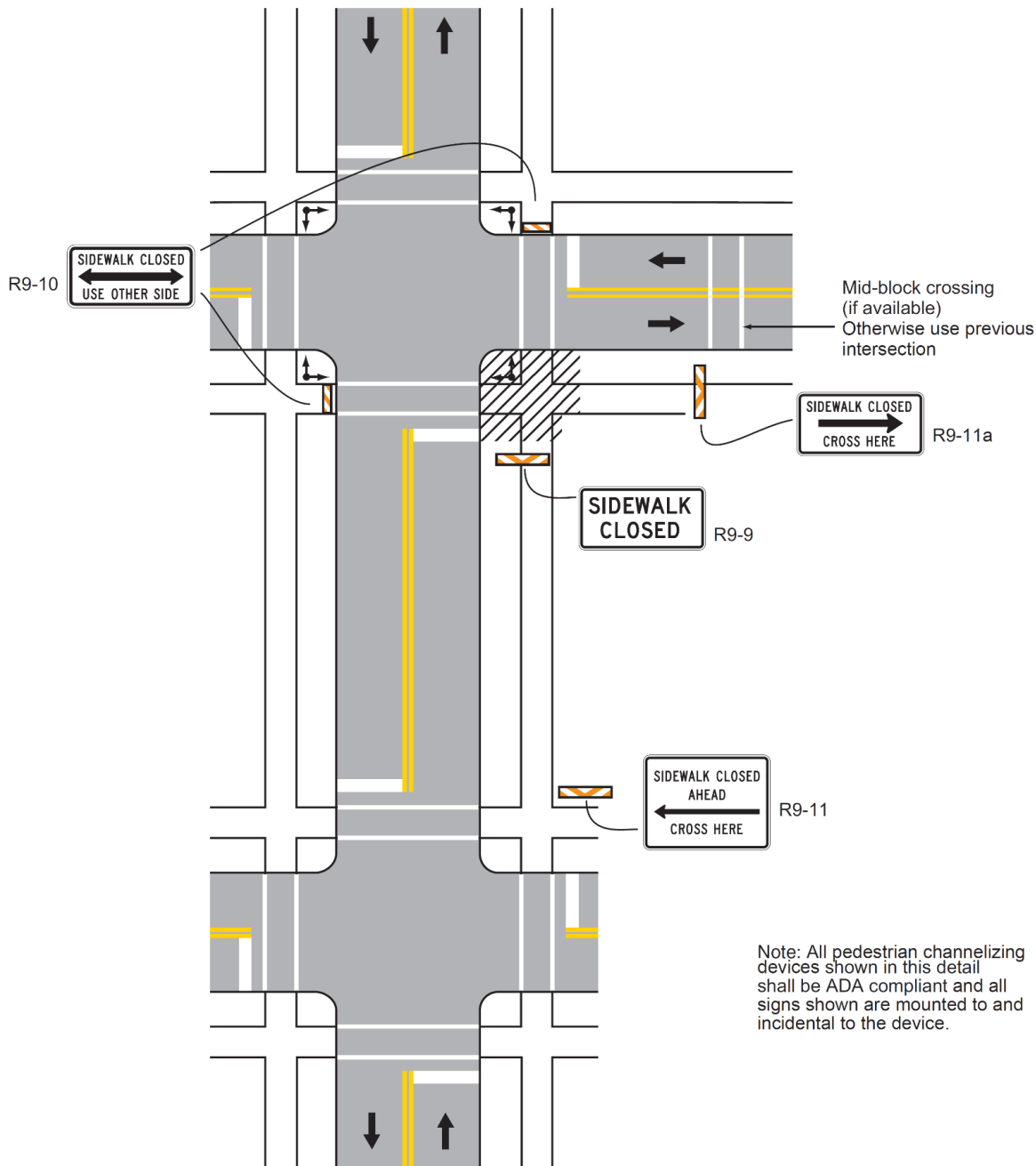
FIGURE 1 Crosswalk Closures and Pedestrian Detours
